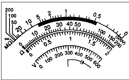
Typical scale (not full size) 210800-4 (210801-4 similar)
