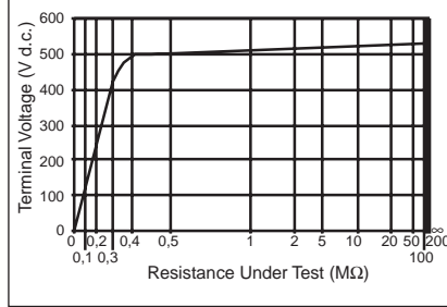
Typical terminal voltage characteristic
