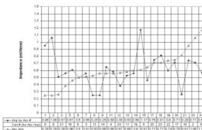
Figure 5. Ascending Impedance.
