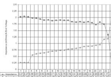
Figure 6. Ascending Impedance compared to Load Test,
